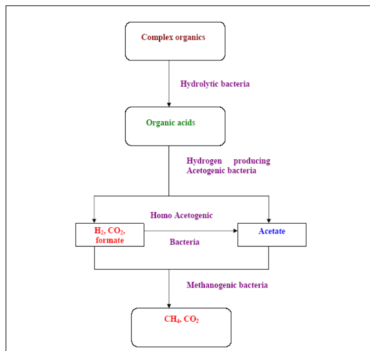
Figure 3. Biogas production process (Omer, 2003)
