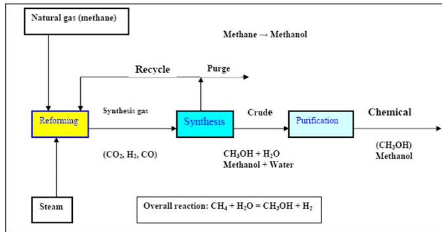
Figure 2. Schematic diagram shows methanol production (Omer, 2006)
