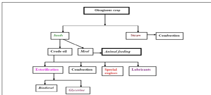
Figure 9. Flow chart of biodiesel production (Omer, 2006)
